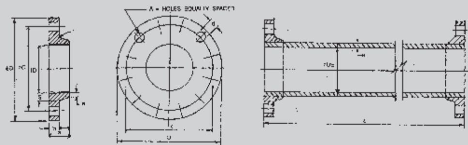
DIMENSIONS OF CENTRIFUGALLY CAST DUCTILE IRON PIPES WITH SCREWED / WELDED FLANGES
